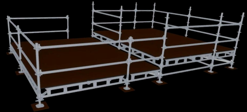
3D SIDE FOH: SOUND: 4m x 3m x 0.3m (W x D x H) LIGHT: 4m x 3m x 0.6m (W x D x H)
